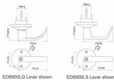
ED8900LQ Lever shown
